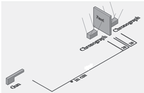
Fig. 4. Chronograph setting up.
