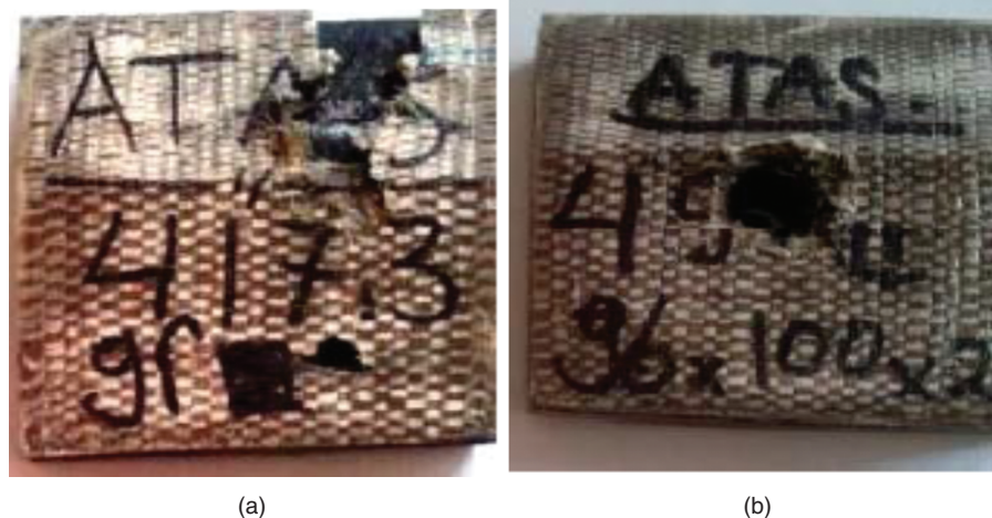
Fig. 5. (a) C 2 specimen (b) C 4 specimen.
