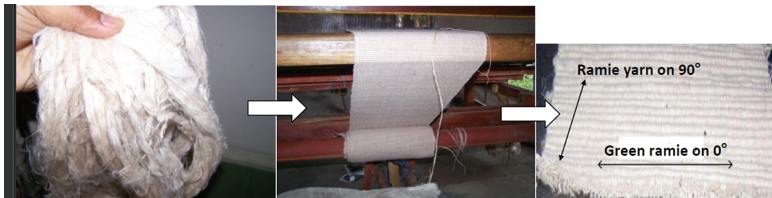
Fig. 1. Processing of ramie.
